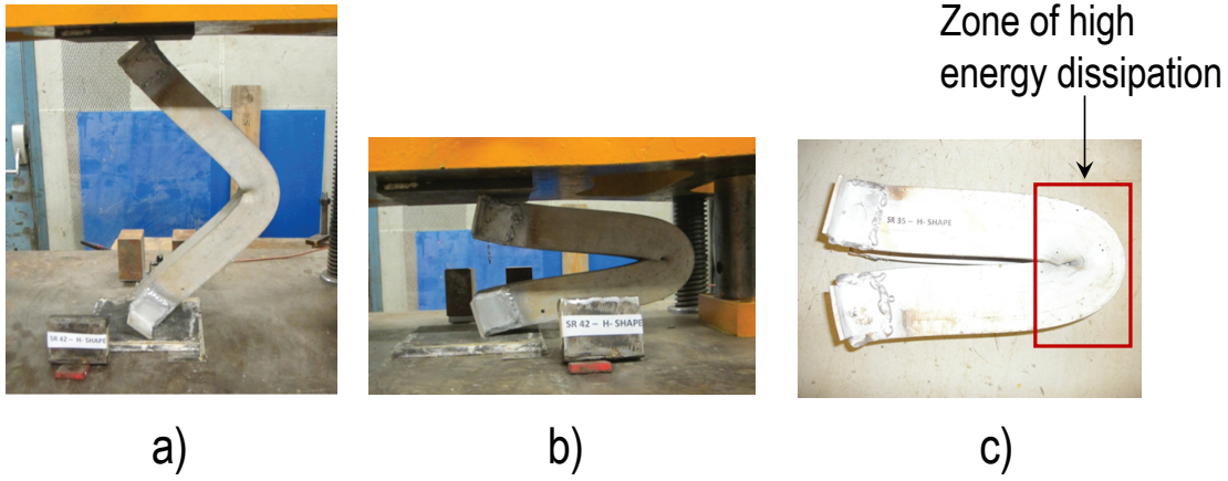
Figure 1: Experiments by Korol and Sivakumaran: a)-b) specimen during the test, and c) final deformation shape of the specimen (Source: Fig. 3 and Fig 7a in Korol Sivakumaran [5]).
