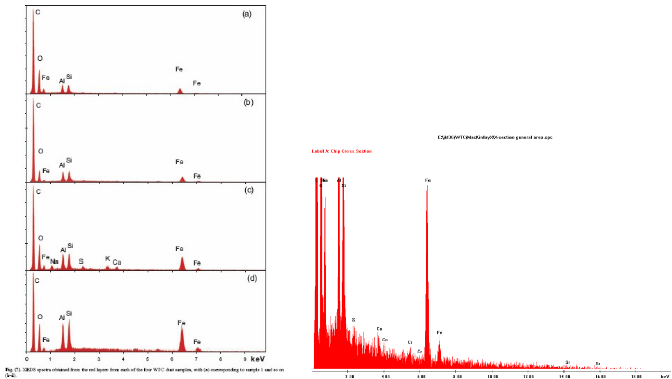
Figure 5. SEMXEDS (beam energy 20 keV) spectra from fresh surfaces of red phase of red/grey chips.
