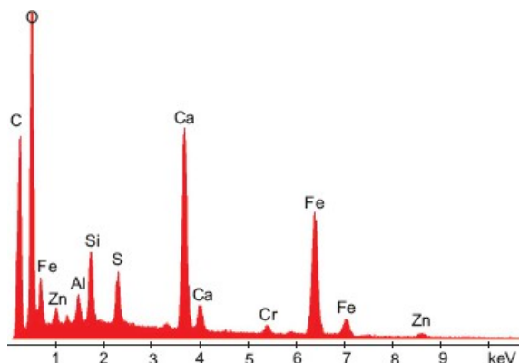
Figure 6. SEMXEDS (beam energy 20 keV) from unbroken chip before soaking in MEK. The calcium and sulfur are likely to originate from contamination with wallboard material (gypsum, calcium sulfate). The signals from zinc and chromium could be from a surface contamination with primer paint.
