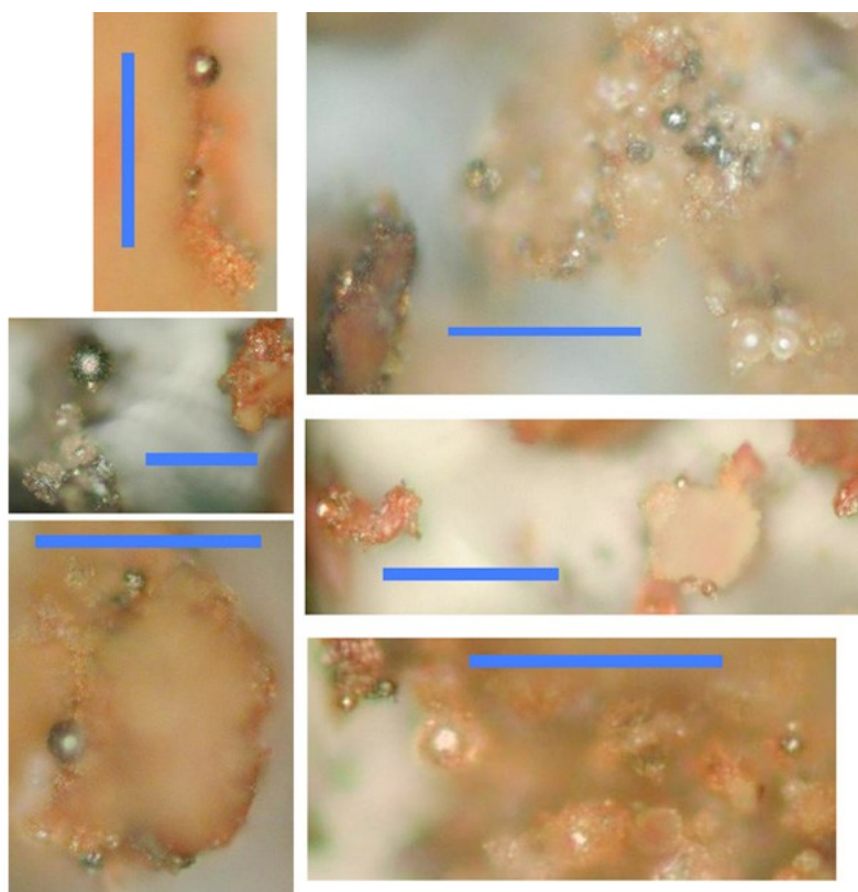
Figure 9. Optical microscope pictures of residues from red/grey chips after reaction in a DSC instrument. 1
